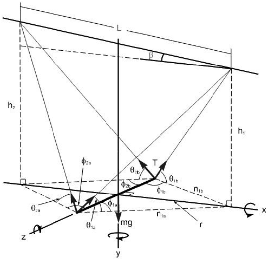
Figure 4: Small body force diagram for a Picavet
