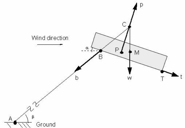
Figure 1: Simple kite model with forces in balance
