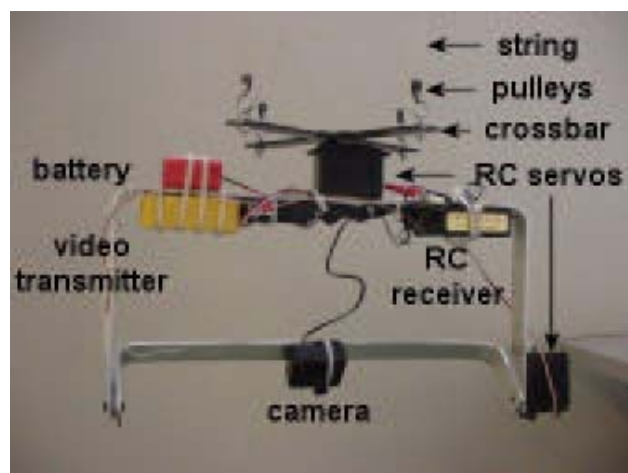
Figure 2: Mechatronic camera rig designed with RC servos, 1/4 mile range 4 mm lens focal length video transmitter and battery pack. Pan and tilt range are both \pm 30^\circ
