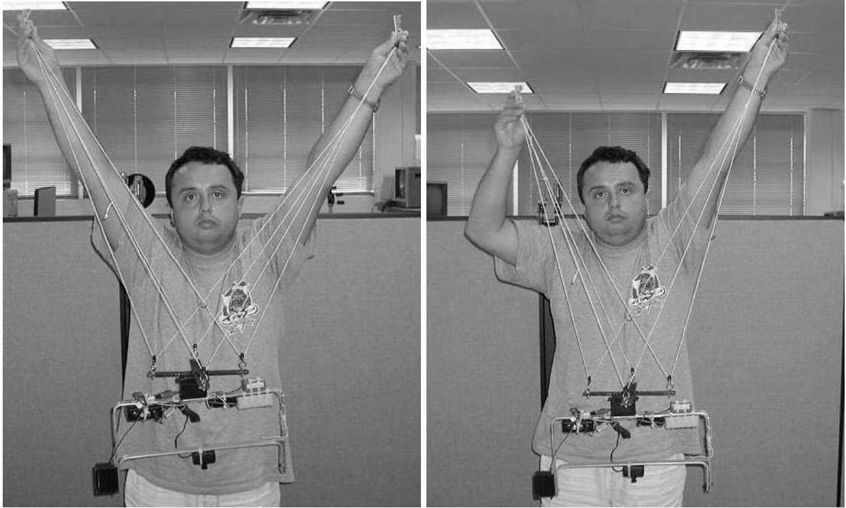
Figure 3: Left: Picavet initial attitude. Right: Attitude is unchanged despite pendulum sway
