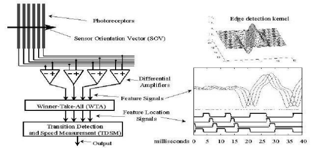
Figure 6: The feature tracker elementary motion detector (EMD).
