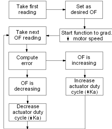
Figure 9: Flow chart of landing control system.
