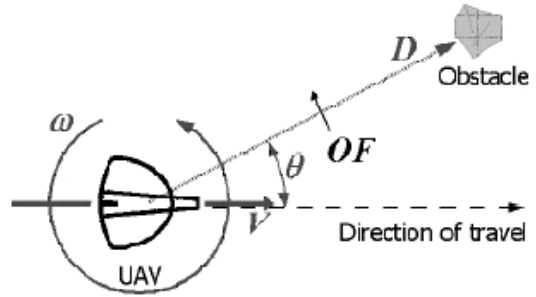
Figure 3: 1D optic flow during MAV flight.
