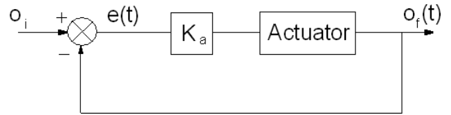
Figure 8: Optic flow control system block diagram.
